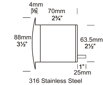
316 Stainless Steel
