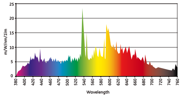
Spectral Power Distribution CMH35MR16/942
