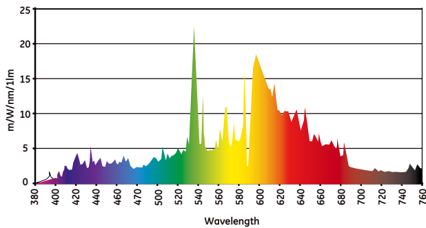
Spectral Power Distribution CMH35MR16/930
