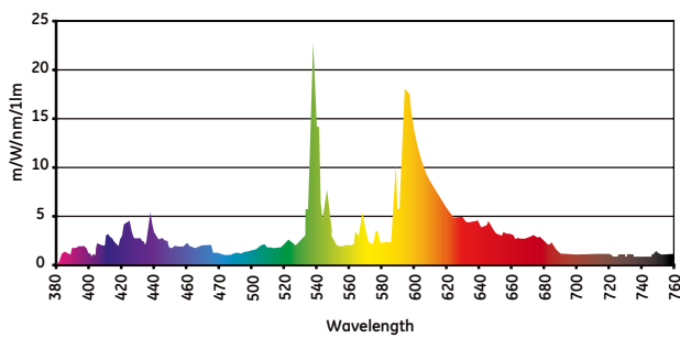
Spectral Power Distribution CMH35MR16/930
